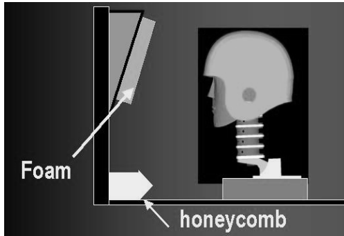
Fig. 5 - Schematic diagram of the mini-sled test configuration.
