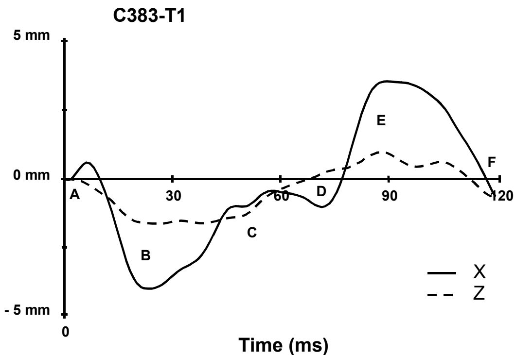
Fig. 4 - Time plot of X and Z relative displacement components of the NDT described in Figure 3.
