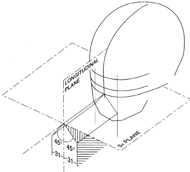
figure 6 .- Breath Deflector Allowance
