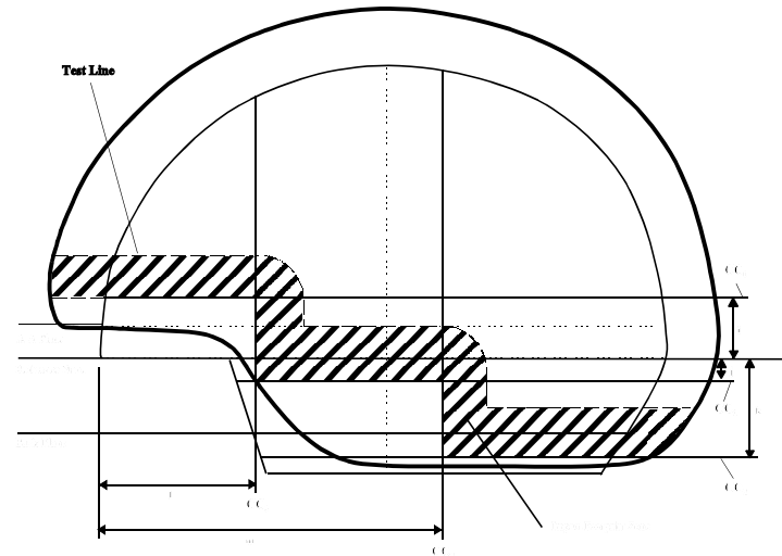
Figure 1a - Extent of Protection Child Helmet
